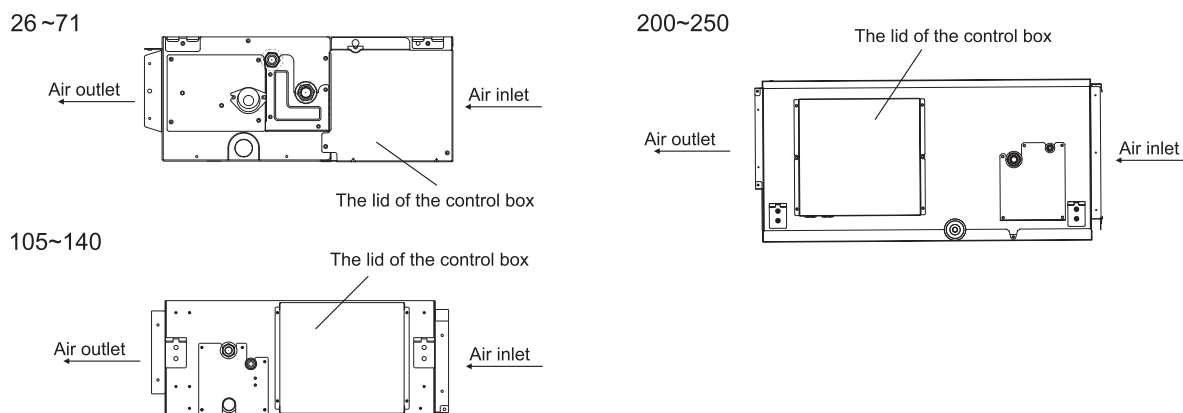
Fig. 6.1 Remove the screws on the control box
