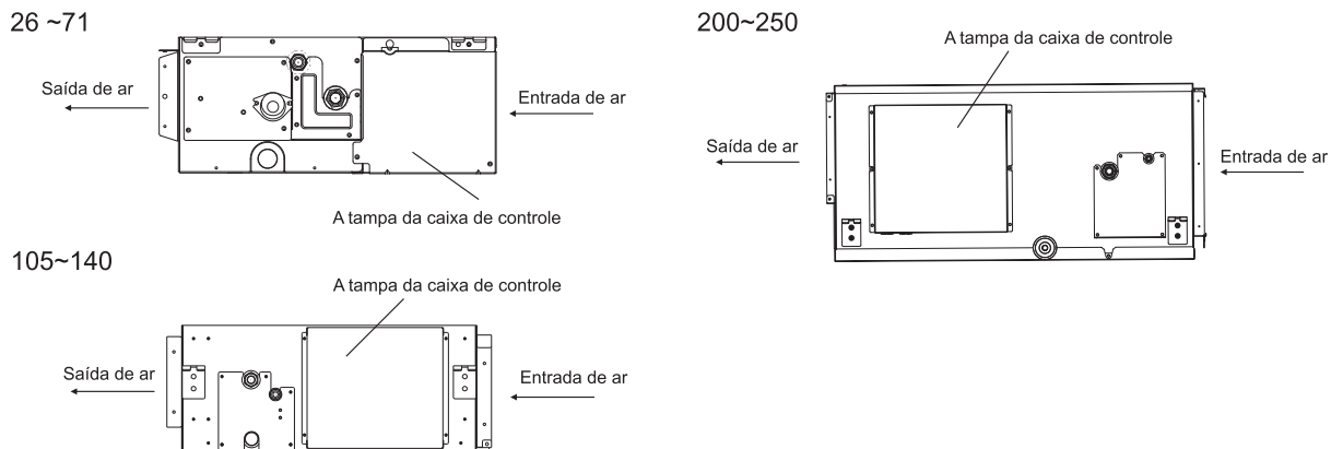
Fig.6.1 Remove the screws on the control box
